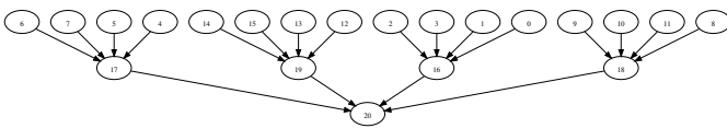
Figure 13. Communication scheme for the BH graph in DT Class A problem.
